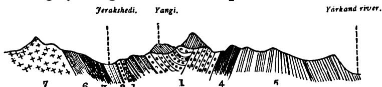
1, Conglomerate; 2, Sandstone; 3, Shales; 4, Black slates; 5, Metamorphic rocks, dark-coloured, with quartzite; 6, Fine-grained gneiss; 7, Unstratified (granitoid) porphyritic gneiss.
