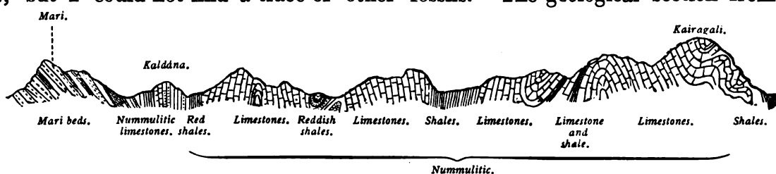
Section from Mari to Kairagali, distance 8 miles.
