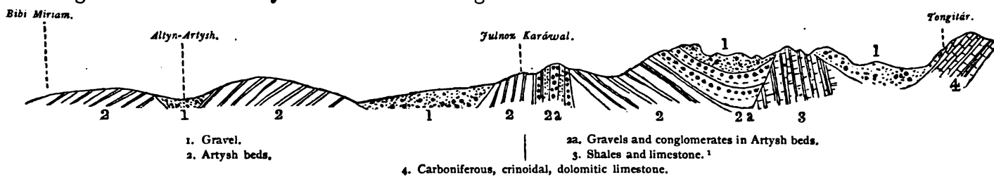
Section from the Káshghar plain to Tongitár, about 25 miles.
